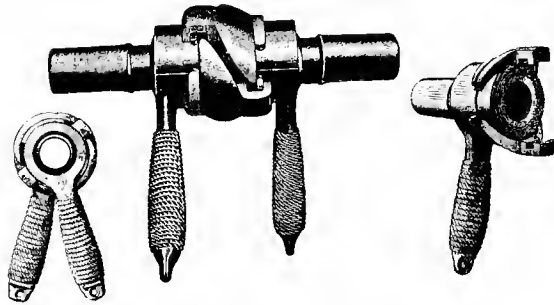
Figs. 2985-2987. THE McELROY STEAM-HOSE COUPLING.
